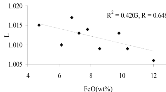
Gambar 1. Plots of lineation (L) and FeO content showing negative correlation
